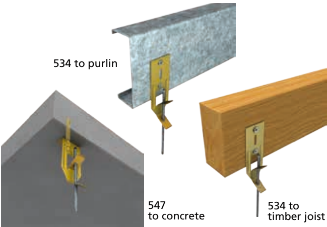
FIGURE 6: HANGER CLIPS
